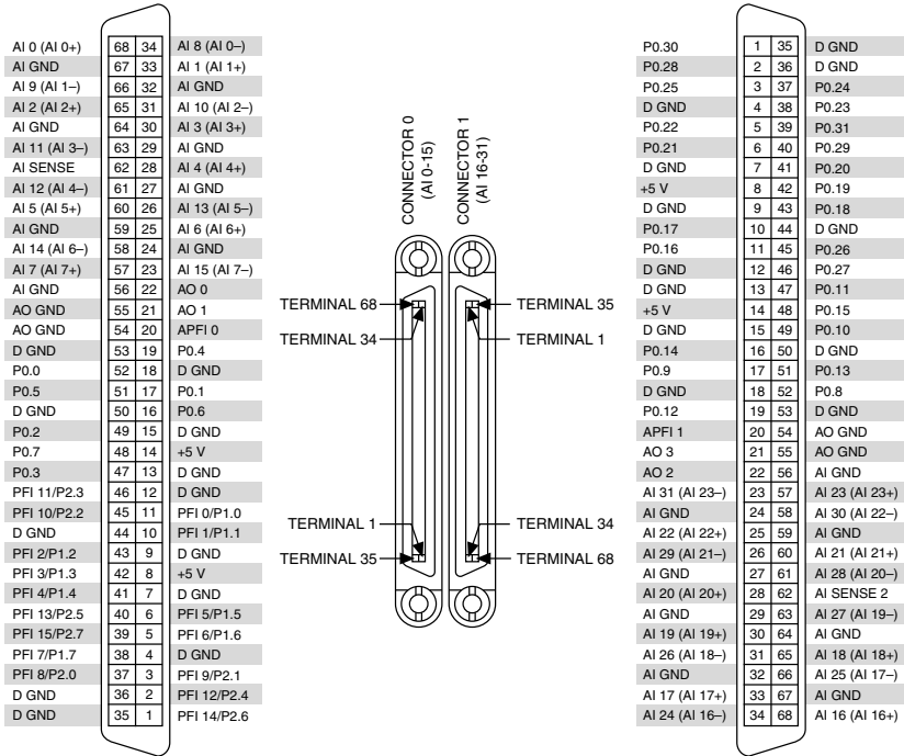
Figure 9. NI PCIe/PXle-6363 Pinout
